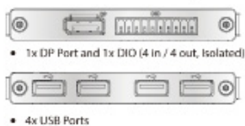
Available Expansion Module Options for Rear Panel
